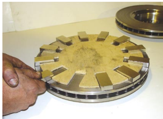
Photo 9: Magnet placement is aided by the jig.
