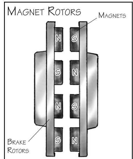
Attracting magnets must face each other exactly on the rotor.
